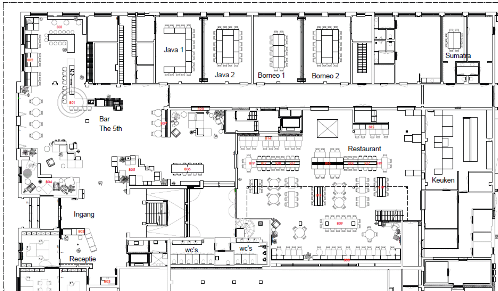
Begane grond 1:200
